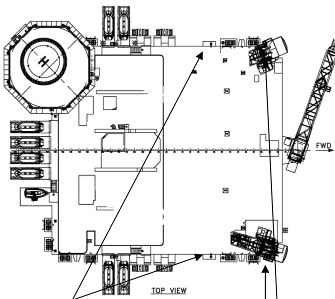
Loading Stations, Hose reel station on Port and stbd side
